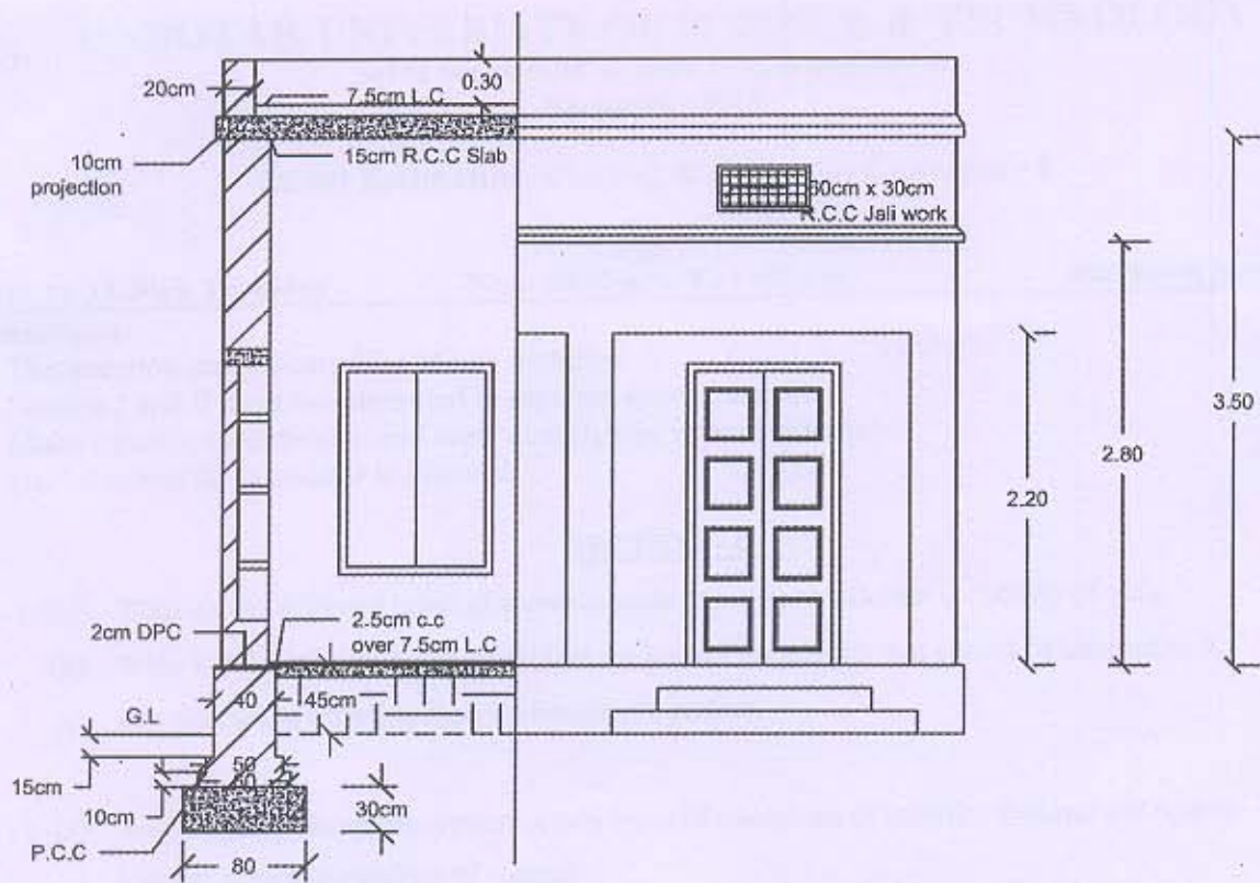
PART SECTIONAL ELEVATION ABC
